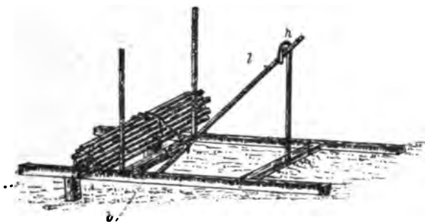
Fig. 158.—Faggot-binder's press.
